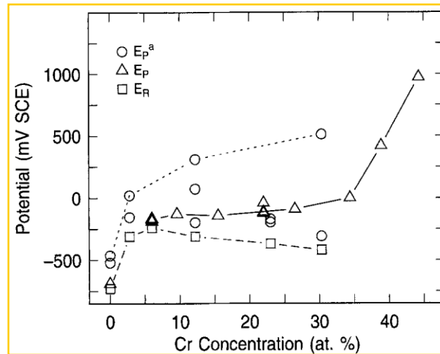
Fig. 4. Pitting potentials for freshly deposited samples, E_{p^a} and aged samples, E_p along with repassivation potentials, E_R for pure Al and AlCr alloys.
