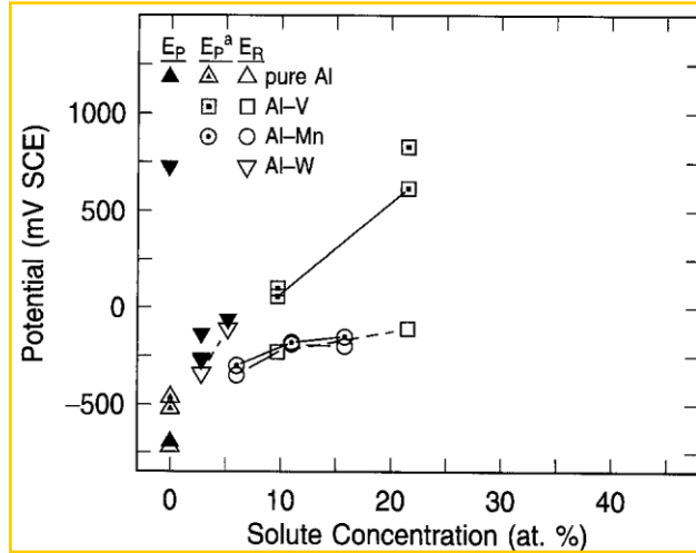
Fig. 3. Pitting potentials for freshly deposited samples, E_{p^a} and aged samples, E_p along with repassivation potentials, E_R for pure Al, AlV alloys, AlMn alloys, and AlW alloys.
