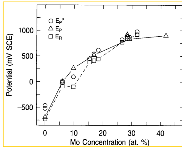
Fig. 2. Pitting potentials for freshly deposited samples, E_p^a , and aged samples, E_p , along with repassivation potentials, E_R , for pure Al and AlMo alloys.
